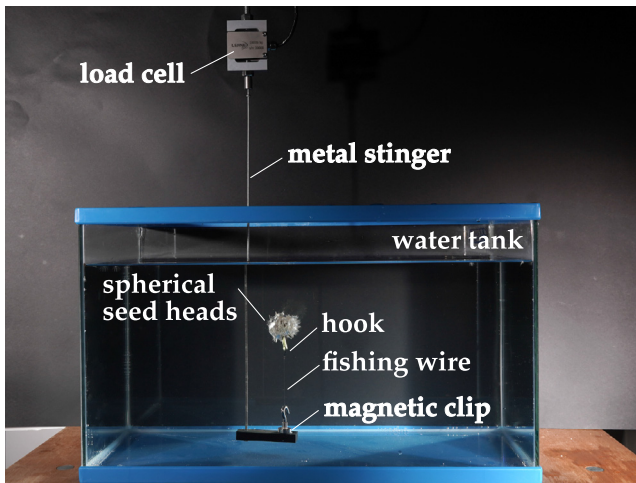
Fig. 4. A photograph of the experimental setup used to measure up-thrust provided by the encapsulated air.
